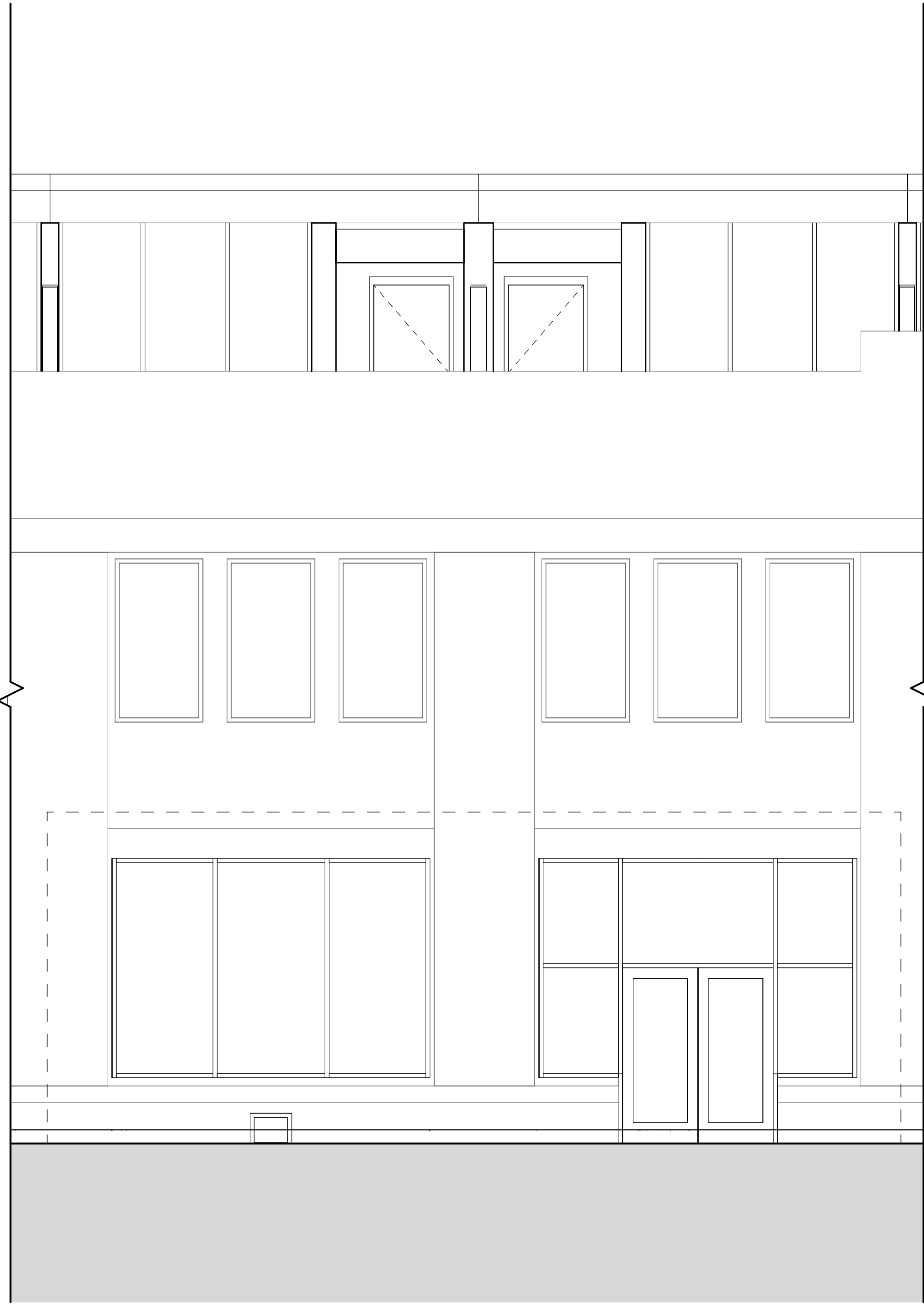
WEST ELEVATION 1/4" = 1'-0"
